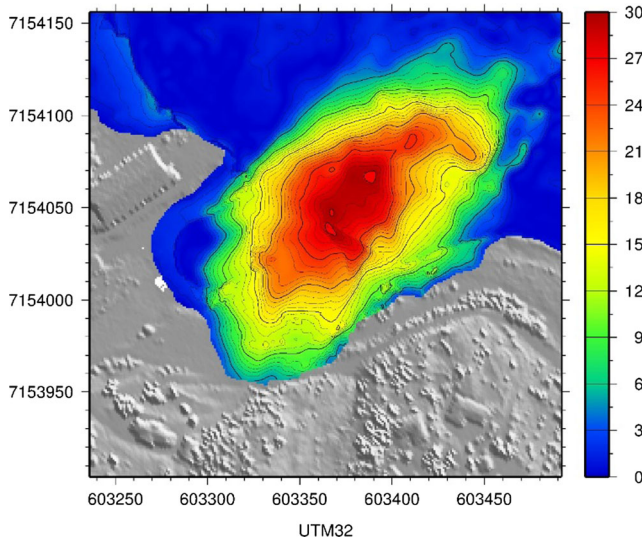
Fig. 4 The initial thickness of the Statland landslide before release based on the difference between the swath bathymetry data collected prior to and after the landslide. The sediment thickness is given in meters. The coordinates are given in UTM zone 32
