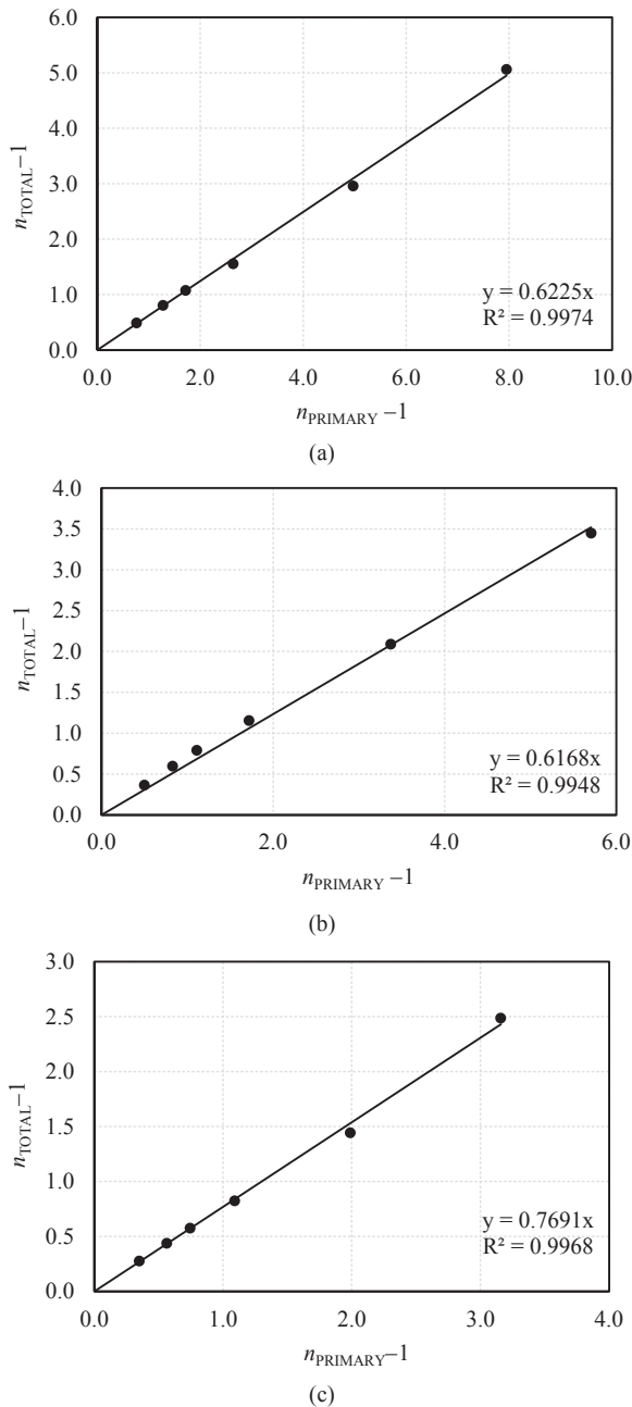
Fig. 8. ( n_{\text{TOTAL}} - 1 ) vs. ( n_{\text{PRIMARY}} - 1 ) plots. (a) ISO; (b) ANIS; (c) A&D.
