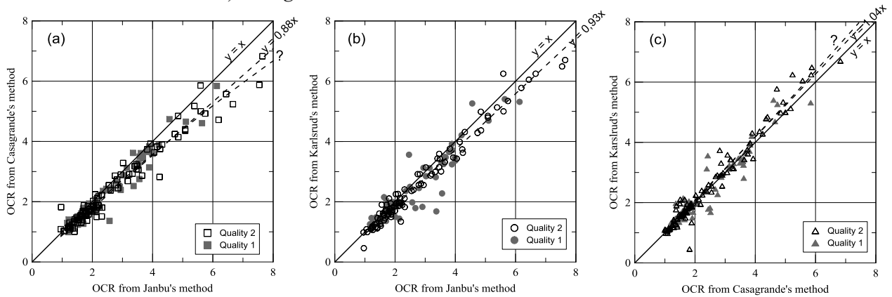
Figure 4. Comparison of OCR' obtained by: a) Janbu's and Casagrande's methods, b) Janbu's and Karlsrud's methods and c) Casagrande's and Karlsrud's methods.
