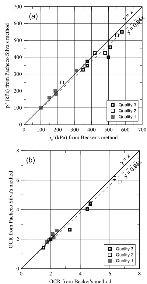
Figure 7. Comparison between a) p_c' and b) OCR from Pacheco Silva's and Becker's methods.
