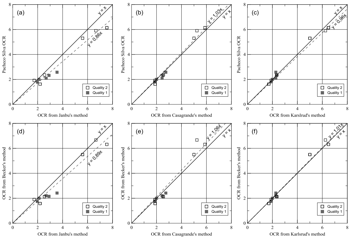
Figure 6. Comparison of OCR obtained by: a) Pacheco Silva's and Janbu's methods, b) Pacheco Silva's and Casagrande's methods, c) Pacheco Silva's and Karlsrud's methods, d) Becker's and Janbu's methods, e) Becker's and Casagrande's and f) Becker's and Karlsrud's methods.
