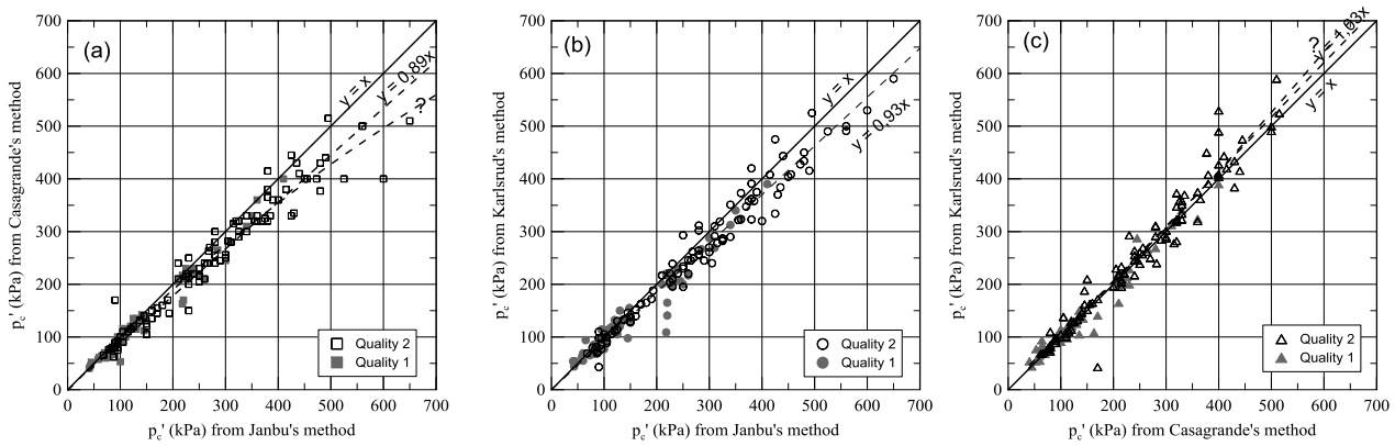
Figure 3. Comparison of p_c' obtained by: a) Janbu's and Casagrande's methods, b) Janbu's and Karlsrud's methods and c) Casagrande's and Karlsrud's methods.
