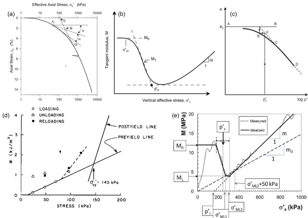
Figure 1. Methods for evaluating p_c' : (a) Casagrande (Holtz and Kovacs, 1981), (b) Janbu (Lunne et al. 2008), (c) Pacheco Silva (Grozic et al. 2003), (d) Becker (Becker et al. 1987) and (e) Karlsrud (Karlsrud and Hernandez-Martinez, 2013).
