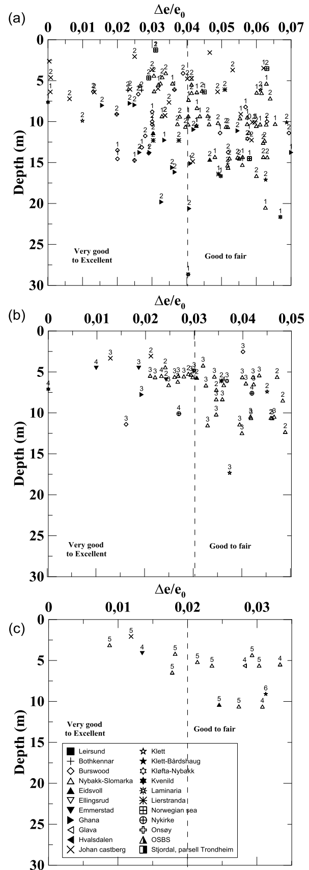
Figure 2. Sample quality for oedometer tests, for OCR between a) 1 and 2, b) 2 and 4 and c) 4 and 6. The OCR is shown over the symbols.
