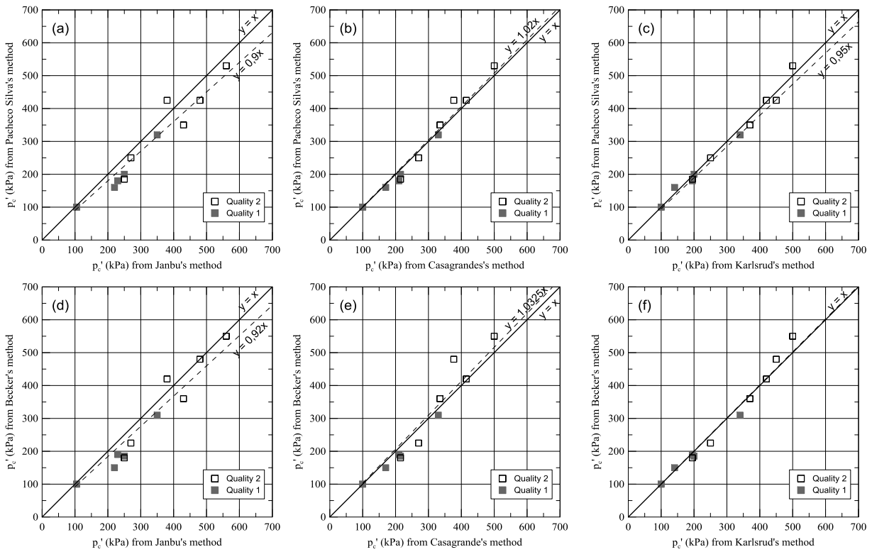
Figure 5. Comparison of p_c' obtained by: a) Pacheco Silva's and Janbu's methods, b) Pacheco Silva's and Casagrande's methods, c) Pacheco Silva's and Karlsrud's methods, d) Becker's and Janbu's methods, e) Becker's and Casagrande's and f) Becker's and Karlsrud's methods.
