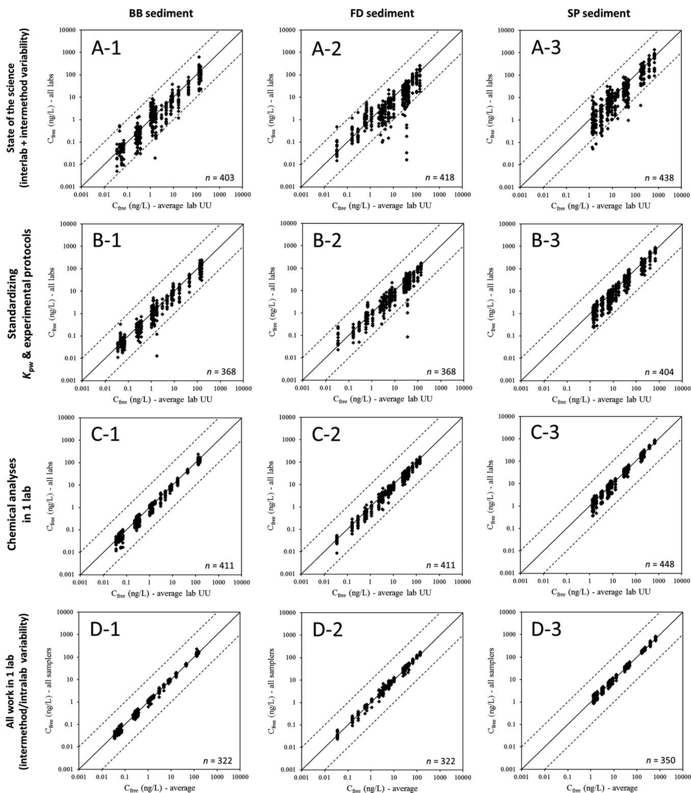
Figure 1. Variability in freely dissolved concentrations ( C_{free} ) determined in three sediments as measured with passive sampling methods (A) when the participants of the interlaboratory comparison followed their own protocols, (B) after standardization of K_{pw} s and experimental protocols, (C) when, in addition to B, all chemical analyses were performed in one laboratory, and (D) when both experiments and analyses with all samplers were performed in one laboratory. Solid lines represent the 1:1 relationships; dashed lines indicate \pm a factor of 10. The n number in each plot indicates the number of data points.
