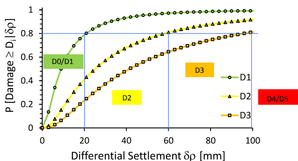
Fig. 6. Fragility curve from Peduto et al. (2019). Threshold at 80% P and definition of different damage classes.
