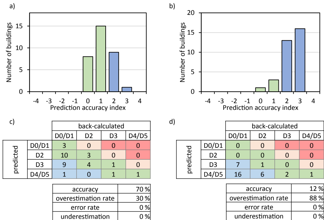
Fig. 14. Kredittkassen case study. The performance analysis has been carried out comparing the damages classes predicted considering the coupled analysis (a, c) and just the impact (b, d). The prediction accuracy index (PAI), as defined by Schuster et al. (2009) (a, b), and the contingency matrix (c, d) have been evaluated.
