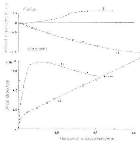
Fig. 5. Shear stress versus horizontal displacement and vertical displacement versus horizontal displacement for two similar samples of low density and very soft in situ hardness sheared at different rates. (Numbers near the curves indicate the sample number.)
