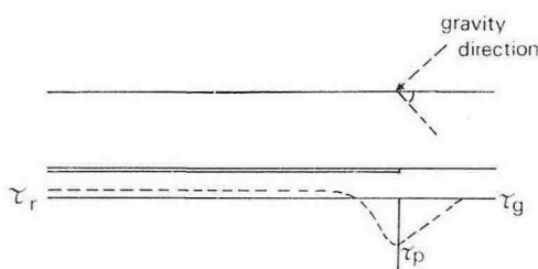
Fig. 6. Schematic of the basal shear stress conditions as a function of distance for a mature slab avalanche with a weak layer exhibiting strain softening. Gravitational body shear stress, peak shear stress and residual shear stress are denoted by \tau_g , \tau_p , \tau_r .
