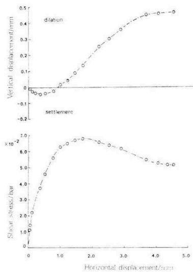
Fig. 3. Typical curves of shear stress versus horizontal displacement and vertical displacement versus horizontal displacement for a sample exhibiting strain softening (sample number 30). Snow properties and test conditions are listed in Table I.
