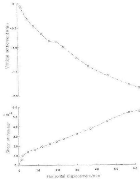
Fig. 2. Typical curves of shear stress versus horizontal displacement and vertical displacement versus horizontal displacement for a sample exhibiting strain hardening (sample number 33). Snow properties and test conditions are listed in Table I.
