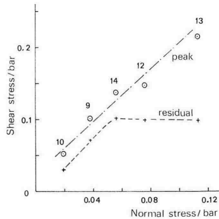
Fig. 4. Estimates of peak shear stress and residual shear stress versus applied normal stress for a group of similar samples. (The numbers near the "peak" data points indicate the sample number.)
