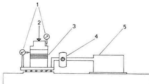
Fig. 1. Diagram of direct simple-shear apparatus. 1. Dial gauges for measurement of horizontal and vertical displacement. 2. Vertical load applied to a top cap over sample. 3. Sample surrounded by reinforced rubber membrane. 4. Load gauge for horizontal force. 5. Gear box containing exchangeable servogear motor.
