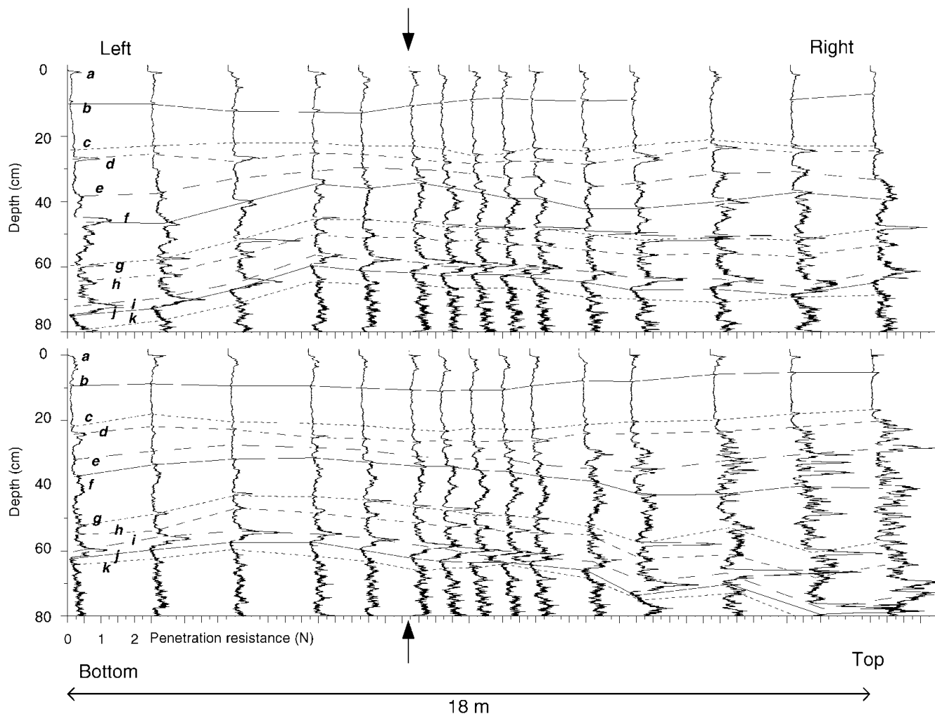
Fig. 4. SMP penetration resistance profiles measured along the two transects indicated in Figure 1. Only the upper 80 cm of the snow cover is shown. Eleven distinct layers are marked with letters a–k and traced with lines through the two transects. Arrows indicate the profile where the two transects cross.
