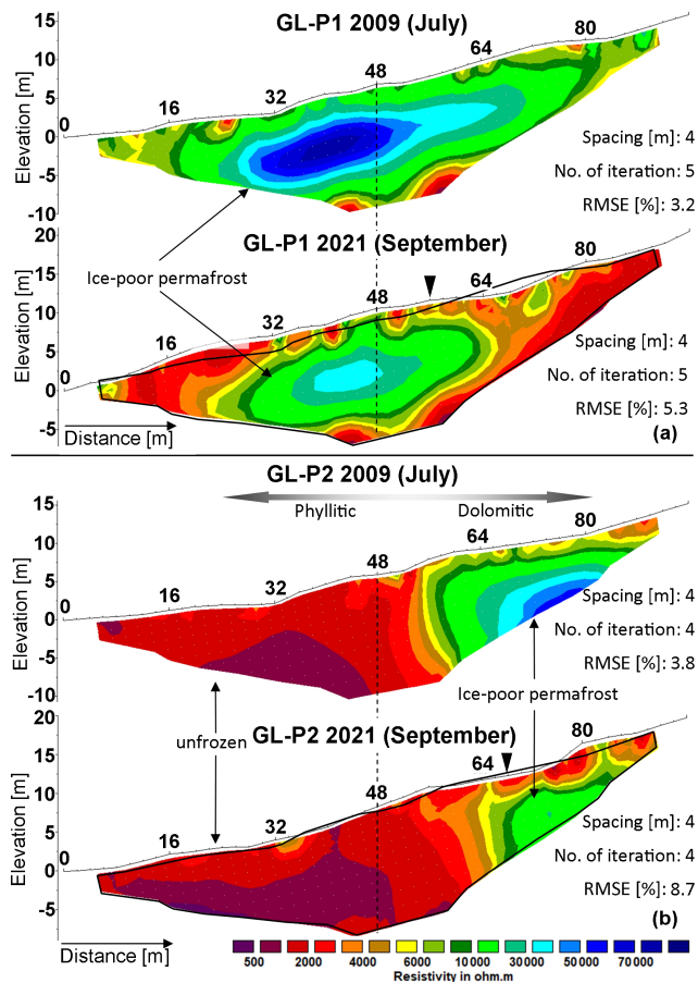
Figure 11. Tomograms of the historical (July 2009) and the repeated (September 2021) profiles GL-P1 and GL-P2 in the Glatzbach catchment. The dashed lines indicate the common center points. The points of intersection of the two perpendicular profiles are indicated by black triangles. The black lines display the outlines of the historical tomograms.
