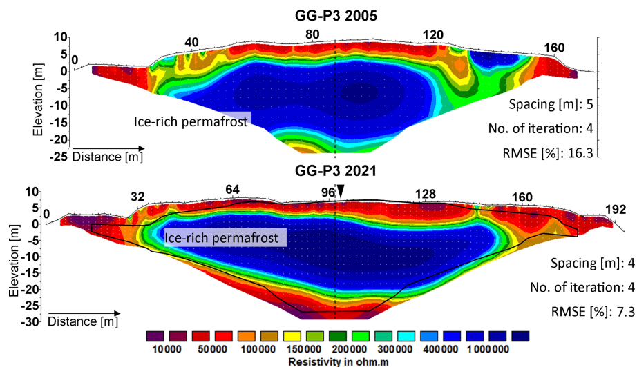
Figure 10. Tomograms of the historical (2005) and the repeated (2021) profile GG-P3 on the Gianda Grischa rock glacier. The dashed line indicates the common center point. The point of intersection with tomogram GG-P2 is indicated by a black triangle. The black line displays the outline of the historical tomogram.
