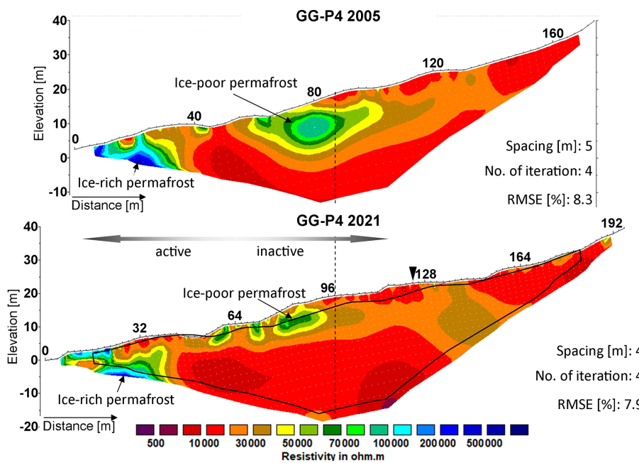
Figure 8. Tomograms of the historical (2005) and the repeated (2021) profile GG-P4 on the Gianda Grischa rock glacier. The dashed line indicates the common center point. The point of intersection with tomogram GG-P1 is indicated by a black triangle. The black line displays the outline of the historical tomogram.
