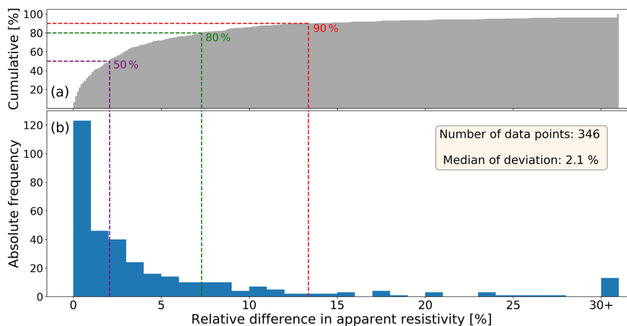
Figure 5. Histogram of the percentage deviation of the measured apparent resistivity for pairwise comparison between quadrupole measurements collected with the new textile electrodes and conventional steel pike electrodes: (a) cumulative distribution and (b) absolute frequency. The dashed lines show defined portions of all data pairs with the corresponding limit of deviation in apparent resistivity.
