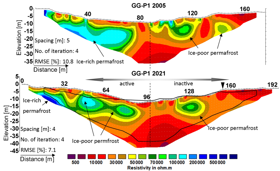
Figure 7. Tomograms of the historical (2005) and the repeated (2021) profile GG-P1 on the Gianda Grischa rock glacier. The dashed line indicates the common center point. The point of intersection with tomogram GG-P4 is indicated by the black triangle. The black line indicates the outline of the historical tomogram.
