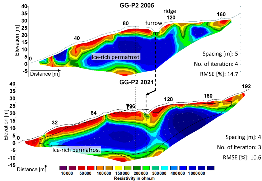
Figure 9. Tomograms of the historical (2005) and the repeated (2021) profile GG-P2 on the Gianda Grischa rock glacier. The thin black dashed line indicates the common center point. The point of intersection with tomogram GG-P3 is given by a black triangle. The thick dashed line and the arrow highlight the observed downgradient shift in furrow. The black line displays the outline of the historical tomogram.
