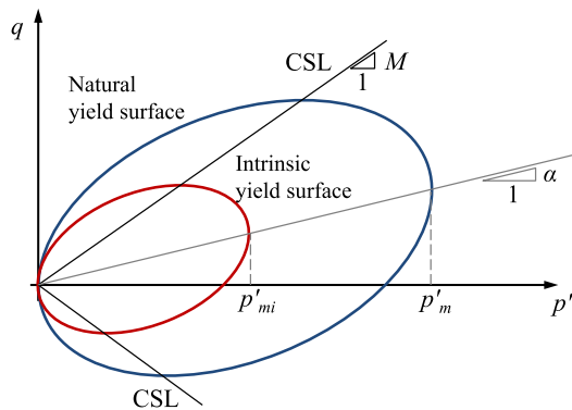
Figure 1. Yield surfaces of the S-CLAY1S model [12]. CSL, critical state line.
