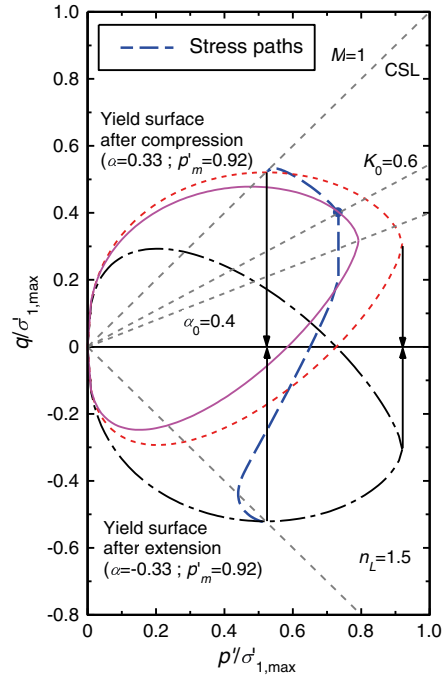
Figure 5. Uniqueness of the critical state line (CSL).
