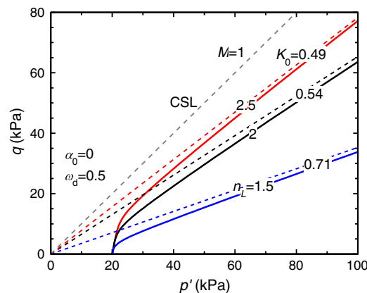
Figure 8. K_{0NC} stress paths. CSL, critical state line.
