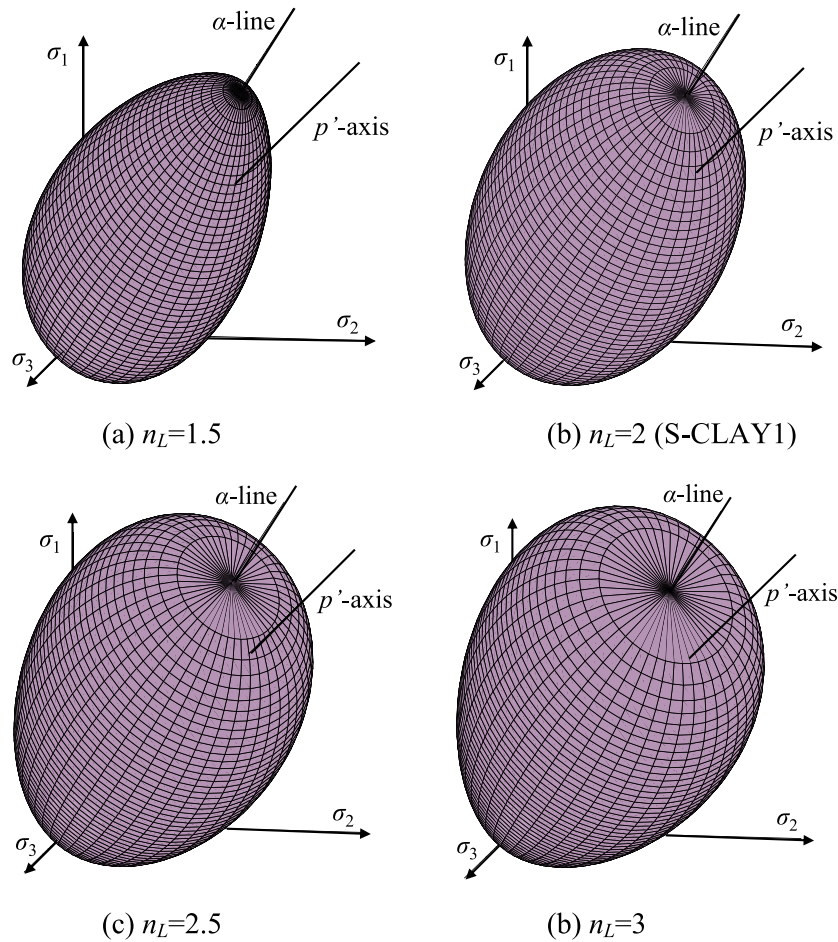
Figure 3. E-SCLAY1S yield surface in general stress space ( M=1.5 , \alpha=0.4 ).
