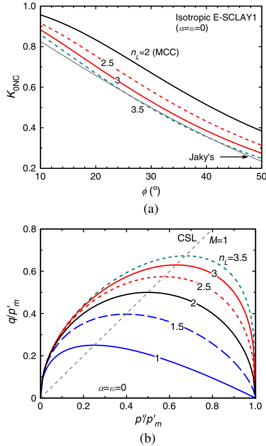
Figure 9. Isotropic E-SCLAY1: (a) K_{0NC} prediction and (b) yield surfaces. CSL, critical state line; MCC, modified Cam clay.
