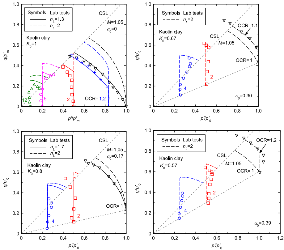
Figure 15. Undrained triaxial stress paths for Kaolin clay (data after [26]). CSL, critical state line; OCR, overconsolidation ratio.
