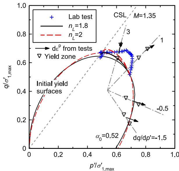
Figure 18. K_0 -consolidated Santa Clara clay (data after [27]). CSL, critical state line.
