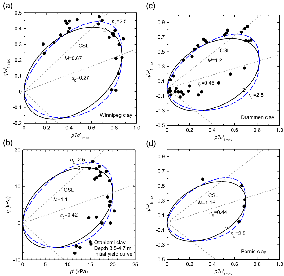
Figure 12. Yield surfaces for several clays: (a) Winnipeg clay (data after [32]), (b) Otaniemi clay (data after [9]), (c) Drammen clay (data after [33]) and (d) Pornic clay (data after [33]). CSL, critical state line.
