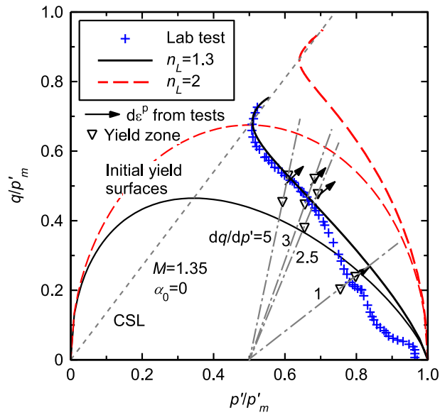
Figure 17. Isotropically consolidated Santa Clara clay (data after [27]).
