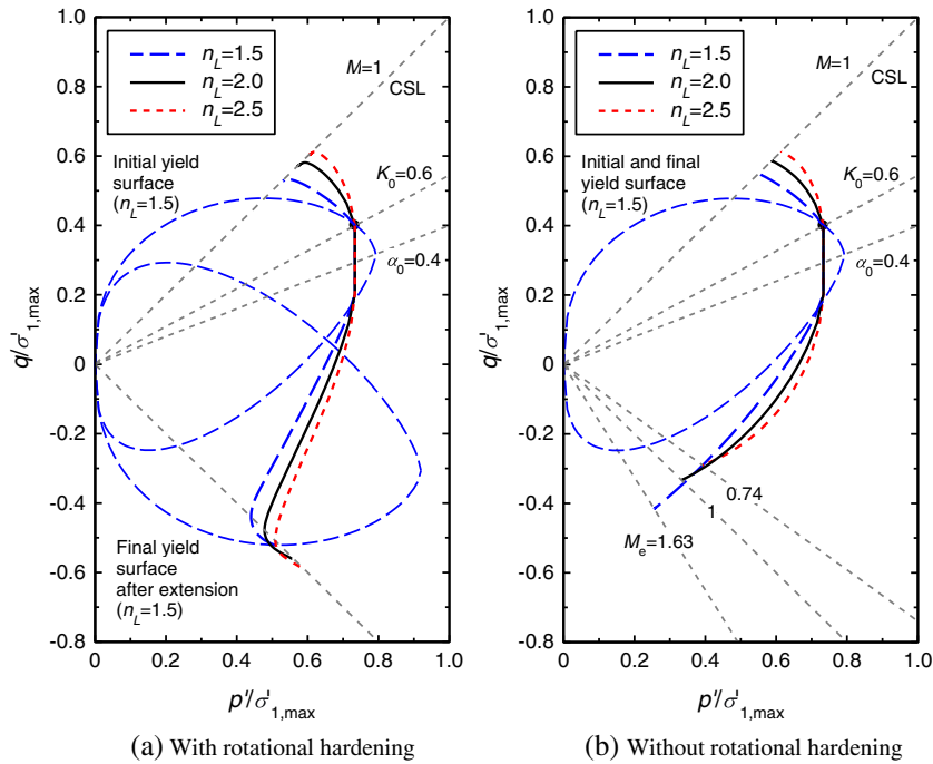
Figure 6. Undrained triaxial stress paths. CSL, critical state line.
