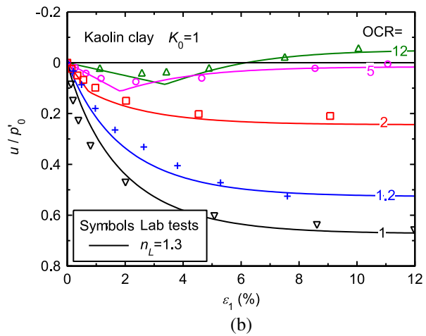
Figure 16. Isotropically consolidated Kaolin clay (data after [26]): (a) stress–strain and (b) excess pore water pressure. OCR, overconsolidation ratio.
