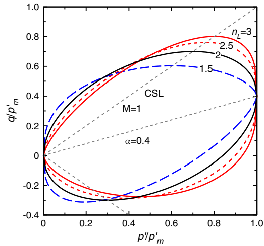
Figure 2. Different shapes of the yield surface for E-SCLAY1S. CSL, critical state line.
