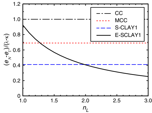
Figure 7. Separation between normal compression line and critical state line. CC, Cam clay; MCC, modified Cam clay.
