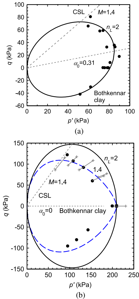
Figure 19. Yield surfaces for Bothkennar clay (data after [29]): (a) K_0 and (b) isotropically consolidated. CSL, critical state line.
