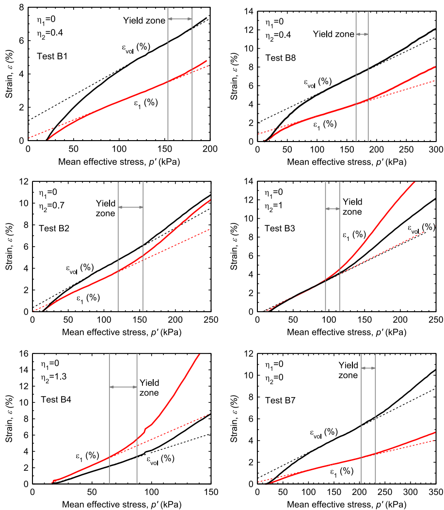
Figure 20. Reinterpretation of yield zone using arithmetic stress scale. Bothkennar clay, isotropically consolidated samples, compression tests (data after [29]).
