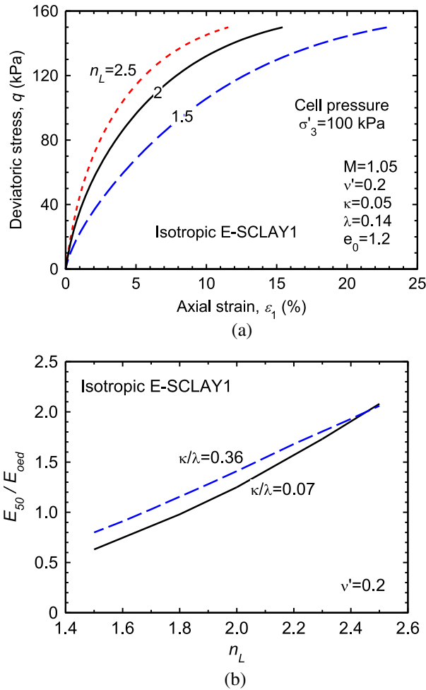
Figure 13. Influence of n_L on soil stiffness: (a) drained triaxial test simulations and (b) stiffness ratio for confined compression and triaxial stress paths.
