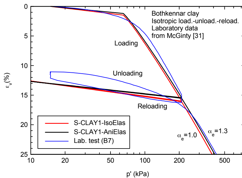
Figure 4. Stress–strain behavior during isotropic loading.
