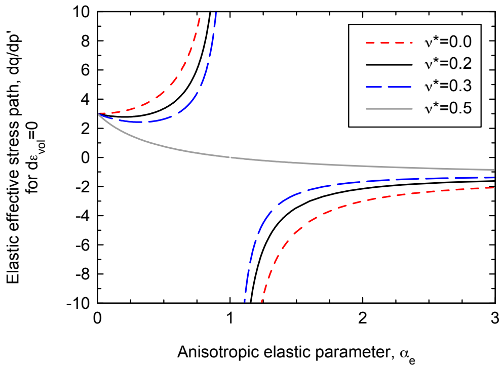
Figure 8. Elastic effective stress path for compression under constant volume ( d\varepsilon_{vol}^e = 0 )
