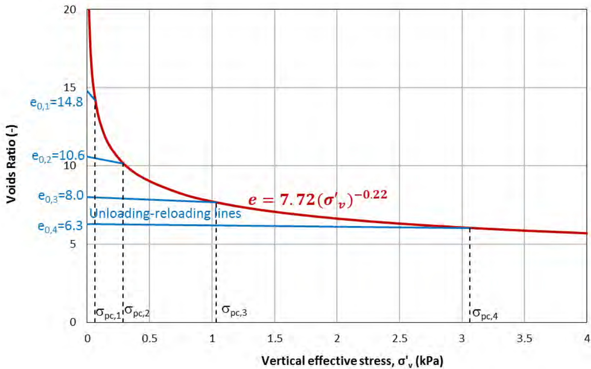
Figure 3 Backbone compressibility curve and unloading–reloading lines for \sigma'_v < \sigma_{pc}
