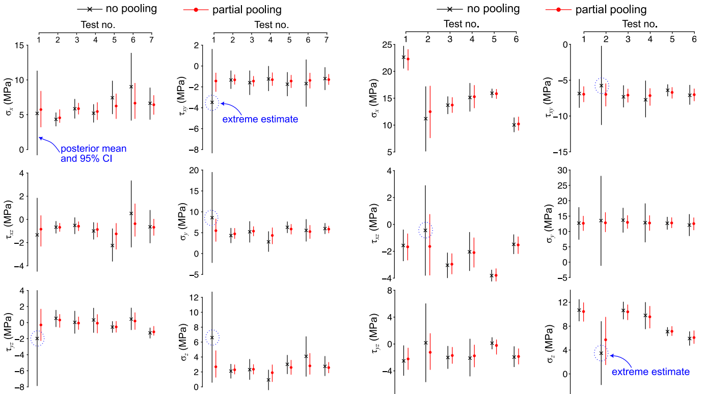
Fig. 5. Posterior estimates of test-specific stress tensors for KA10X OC tests from the no and partial pooling models.
